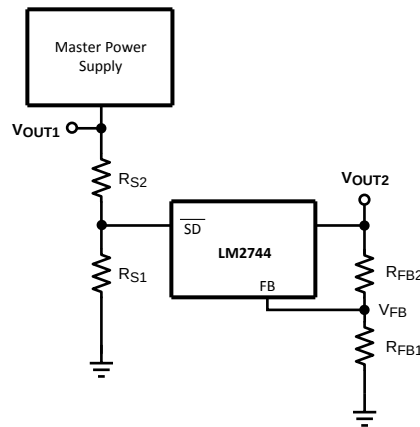
Figure 24. Sequencing Circuit
